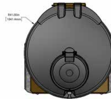
4.5YD SURFACE MOUNTED SHOWN WITHOUT CONCRETE RING
